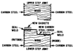
JOINT DETAIL DOT SPECIFICATION 21PF-1A OVERPACK
